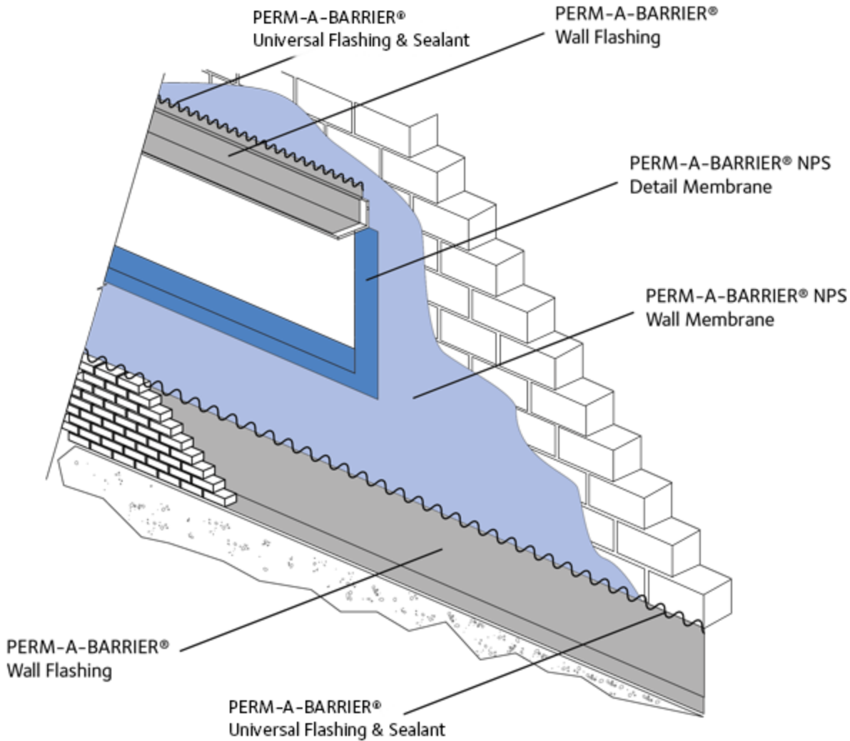
Typical Air and Vapor Barrier Application
