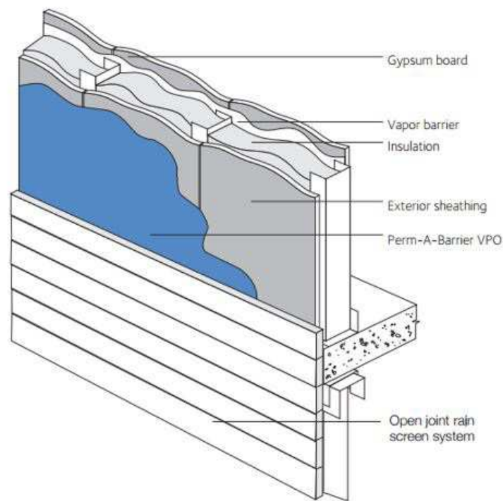
Figure of Perm-A-Barrier® VPO typical vapor permeable air barrier application. Consult GCP for climate specific details.
