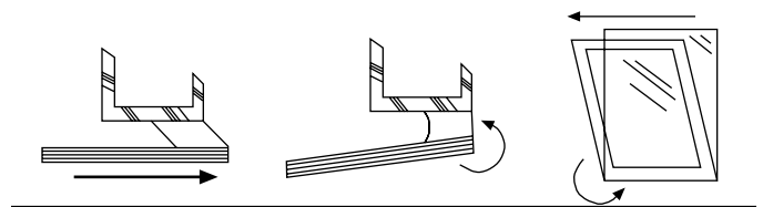
Figure 2: Movement from thermal expansion and contraction and/or glass rotation
