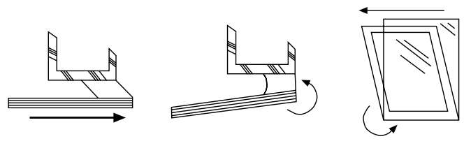
Figure 2: Movement from thermal expansion and contraction and/or glass rotation.
