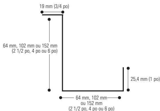
Coin J-L
