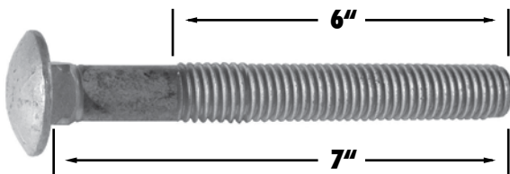
½"-13 x 7" overall length – 6" Thread Length
