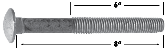
½"-13 x 8" overall length – 6" Thread Length
