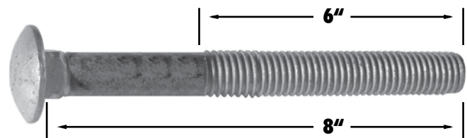
½"-13 x 8" overall length – 6" Thread Length
