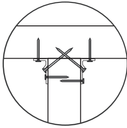
Joist Hanger
