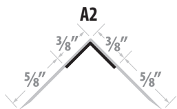
A2 Inside Tape-On Cornerbead
