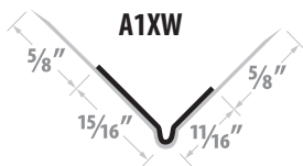
A1XW Tape-On Odd Leg Outside Corner
