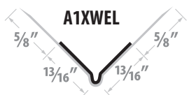
A1XW EL Tape-On Extra Wide Outside Corner
