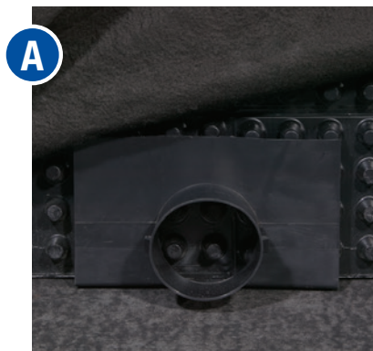
6" Sideout Connector attached to CCW MiraDRAIN HC
