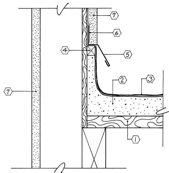
DETAIL 21, PARAPET WALL / COUNTERFLASHING
