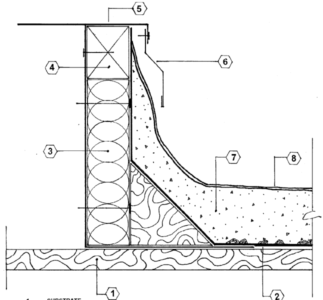
DETAIL 33, PRE-FAB METAL A/C CURB EXISTING BUR
