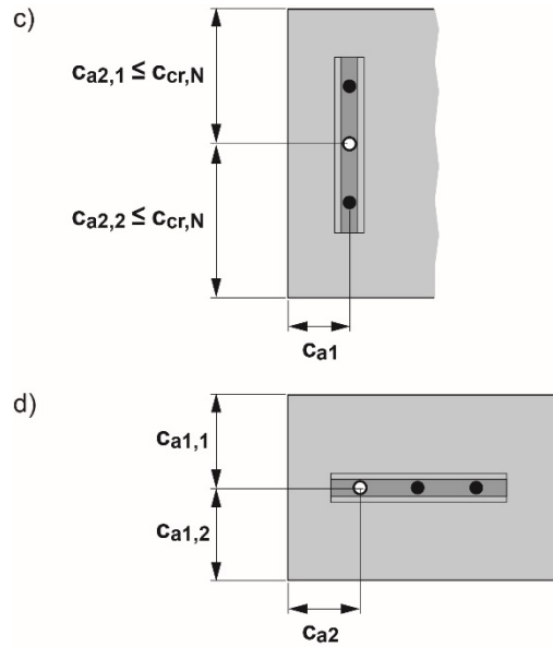
Figure 4-10: Anchor channel at a corner of a concrete member
