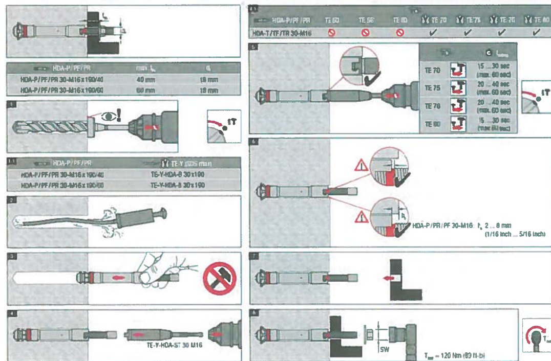
FIGURE 8—INSTALLATION INSTRUCTIONS HDA-P/PF/PR M16
