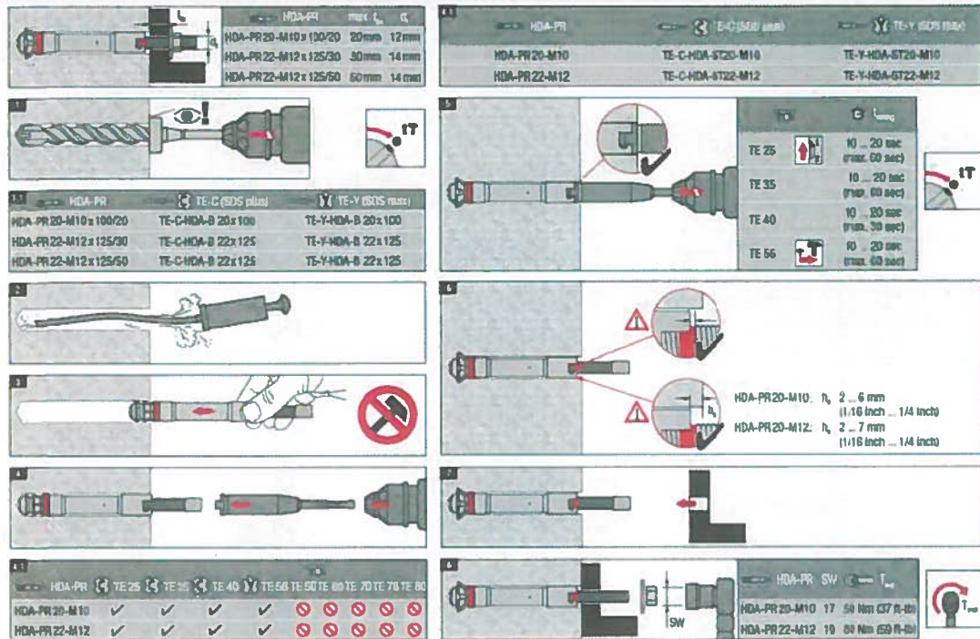
FIGURE 7—INSTALLATION INSTRUCTIONS HDA-PR M10 AND HDA-PR M12
