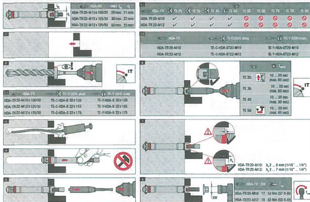
FIGURE 12—INSTALLATION INSTRUCTIONS HDA-TR M10 AND HDA-TR M12
