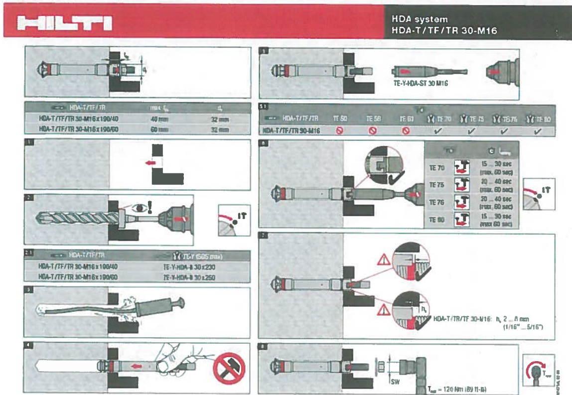
FIGURE 13—INSTALLATION INSTRUCTIONS HDA-T/TF/TR M16
