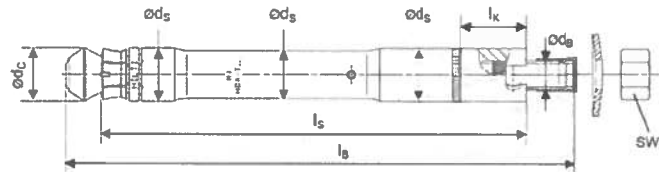
FIGURE 3—HDA DIMENSIONS
