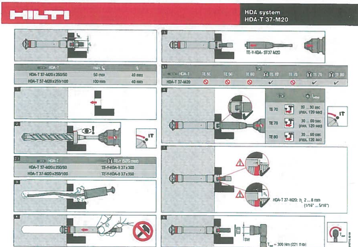
FIGURE 14—INSTALLATION INSTRUCTIONS HDA-T M20
