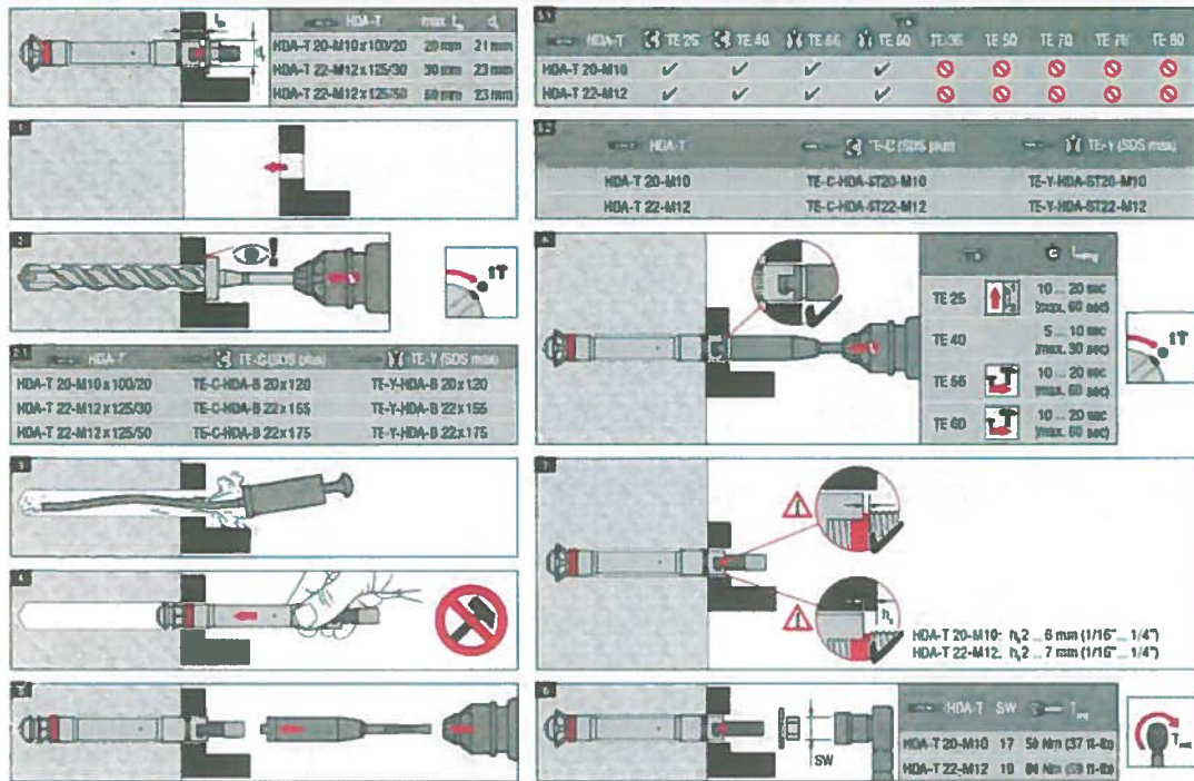
FIGURE 11—INSTALLATION INSTRUCTIONS HDA-T M10 AND HDA-T M12
