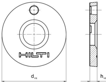
Sealing washer
