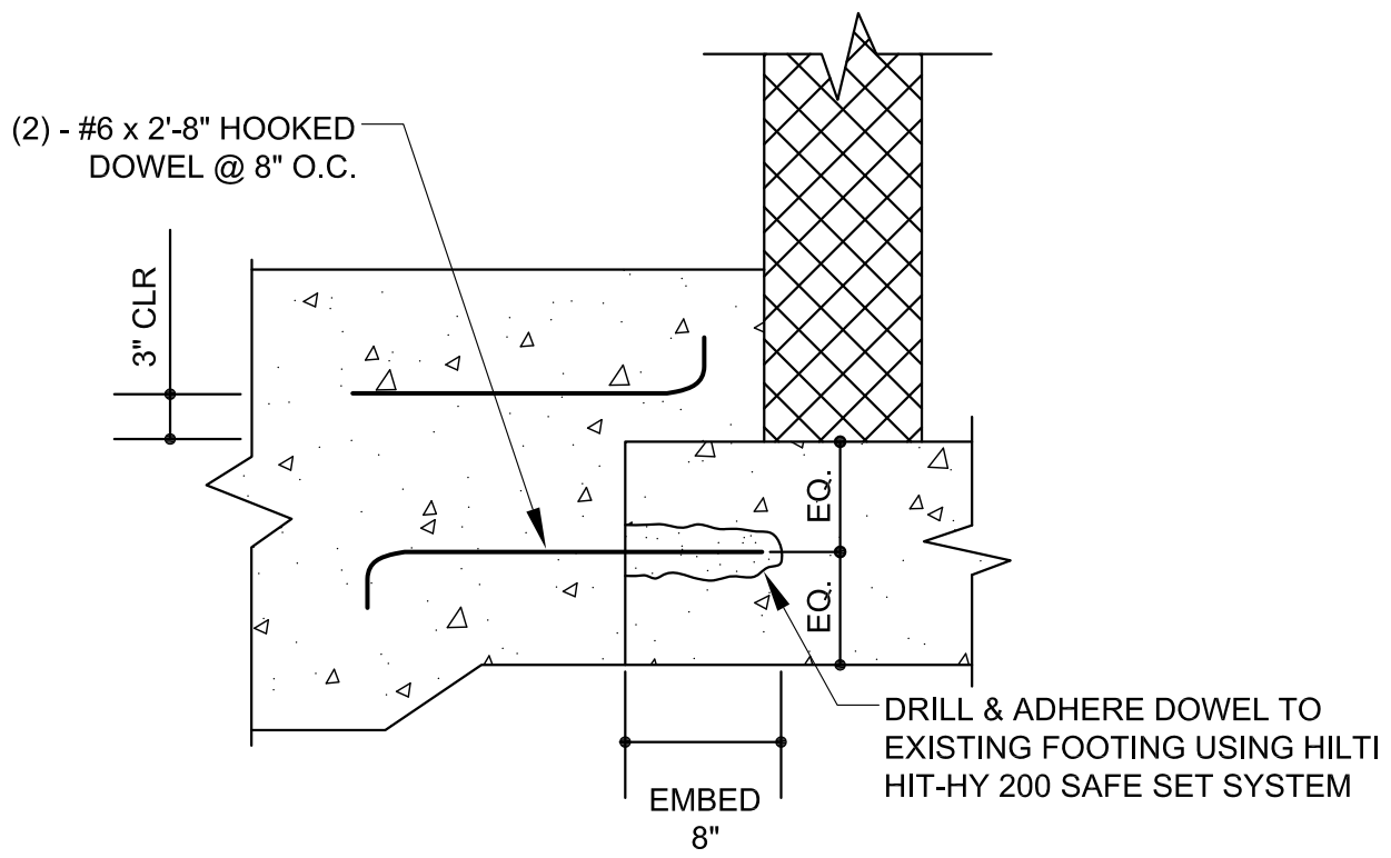
HY 200 TYPICAL DETAIL
