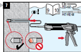
FIGURE 7—MANUFACTURER'S PRINTED INSTALLATION INSTRUCTIONS (MPII) (CONTINUED)
