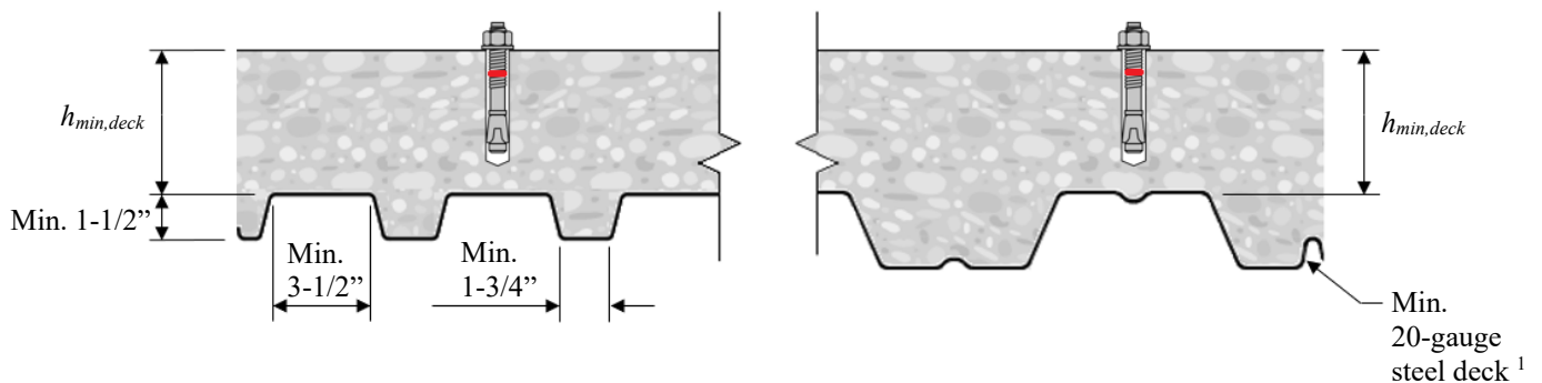
FIGURE 5F—KB-TZ2 IN THE TOP OF CONCRETE FILLED PROFILE STEEL DECK ASSEMBLIES
