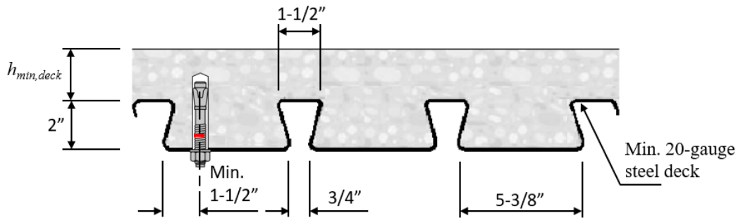
FIGURE 5D— KB-TZ2 IN THE SOFFIT OF CONCRETE FILLED PROFILE STEEL DECK ASSEMBLIES – 2" DOVETAIL DECK
