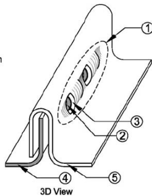
3e. Vercor VSC 2 Connection for use with PLB only
