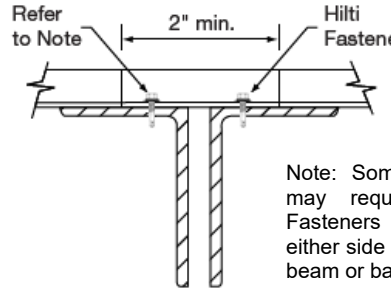
3b. Steel Deck Endlap Condition
