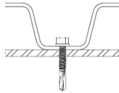
3a. S-MD 12-24 x 1 5 / 8 or S-RT5+ M9 Fastener Attachment of Steel Deck to Frame
