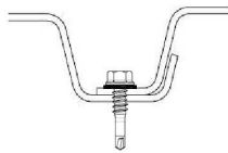
3c. Sidelap Connector with B Deck
