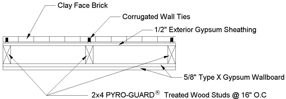
Figure 2 - UL Design U302
