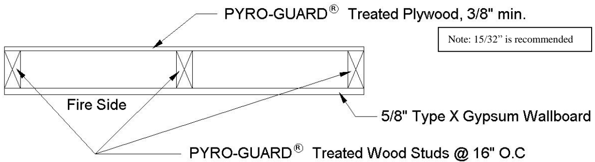
Figure 6 - Fire Separation Distance > 5'-0"
