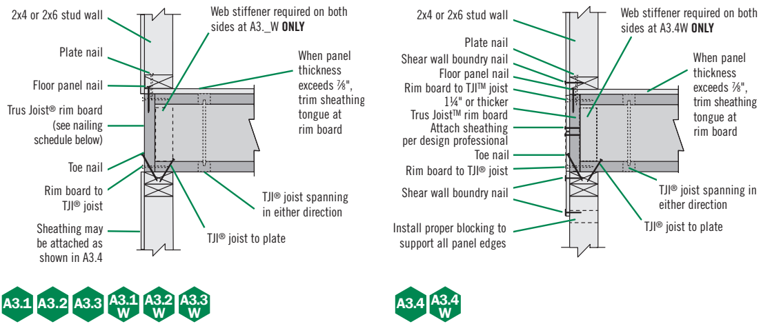
Rim Board Installation Detail (1)(2)(3)
