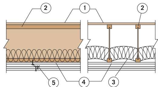
Typical resilient channel and gypsum board attachment
