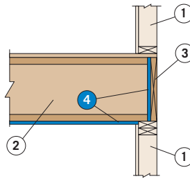
Joists Perpendicular to Wall
