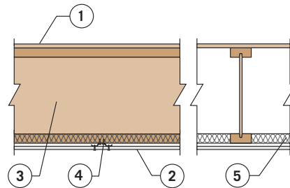
Typical detail for butt joints perpendicular to framing members
