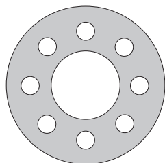
300 LB. Full face
