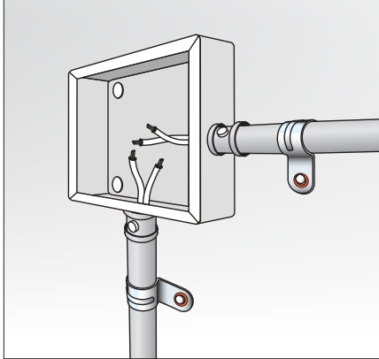
Junction Box / Panel Boards
