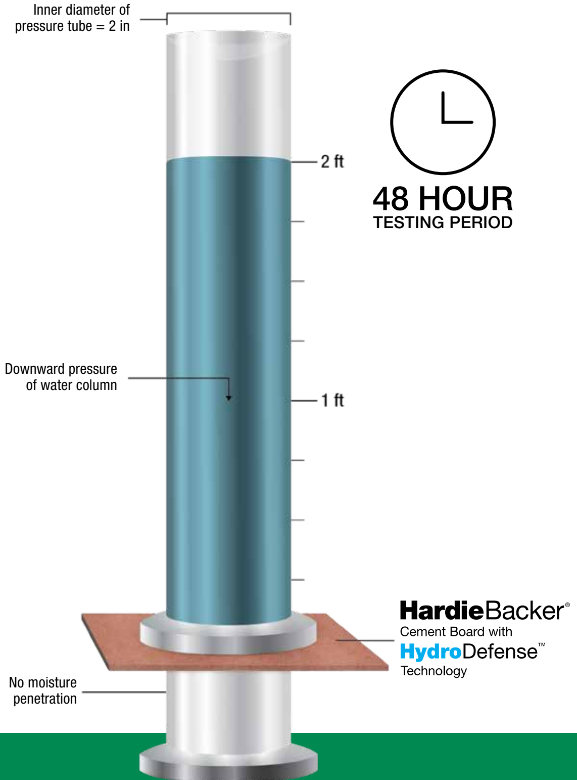
Graphic Representation of ANSI A118.10 Waterproofness Test
