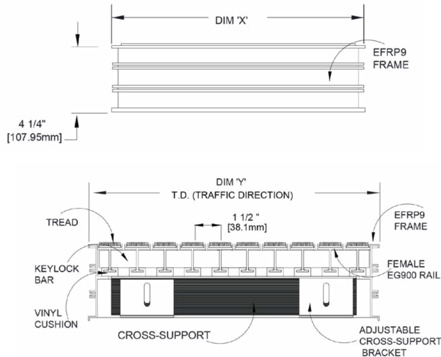
ACTIV-GRATE 900 SERIES INSERTS
