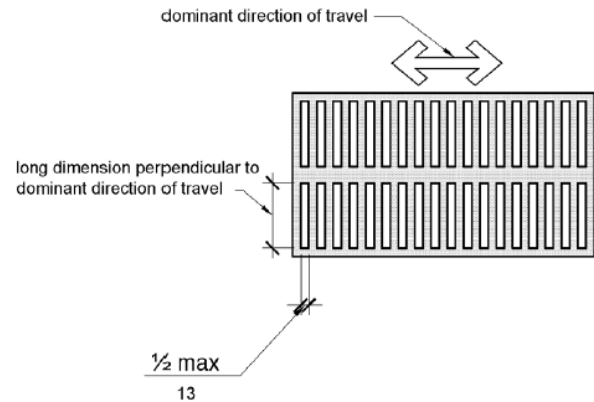
All of JL's tread selections provide less than 1/4" vertical change above the level of the frame and tread rail which are typically installed flush with the floor. Figure 302.3 Elongated Openings in Floor or Ground Surfaces
