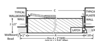
1 1/2 HOUR WALL
