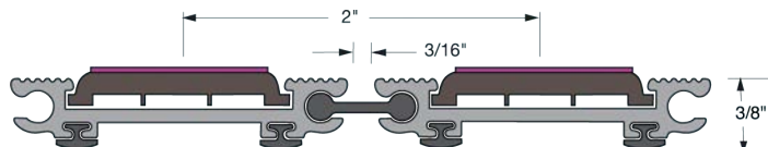
Cross-section: EM704 Premium Carpet Tread
