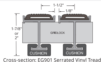
Cross-section: EG901 Serrated Vinyl Tread
