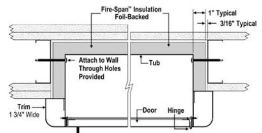
This view is for metal or wood framing installation
