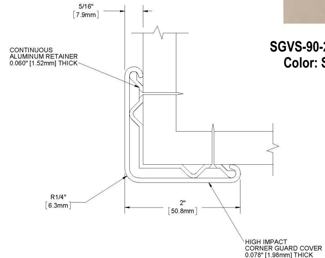
Example of Installation - Cornerguard
