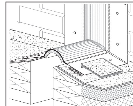
STYLE EJ PF-19 TRANSITION VERTICAL INSIDE CORNER
