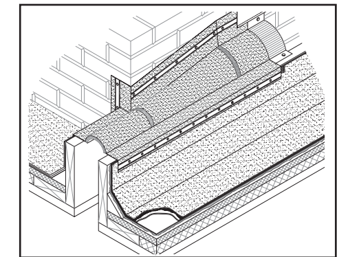
STYLE EJ/WC FF-25 TRANSITION ROOF/WALL TO ROOF/ROOF
