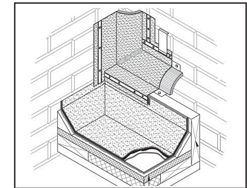
STYLE EJ/WC PF-28 TRANSITION VERTICAL INSIDE CORNER
