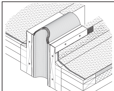
STYLE CF EG-1 TRANSITION RR VERTICAL OUTSIDE CORNER
