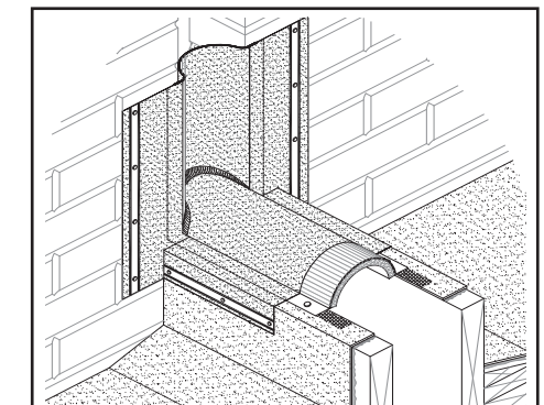
STYLE EJ/WC EG-29 TRANSITION RR VERTICAL INSIDE CORNER
