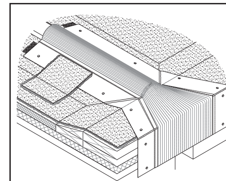
STYLE EJ FF-17 TRANSITION GRAVEL STOP
