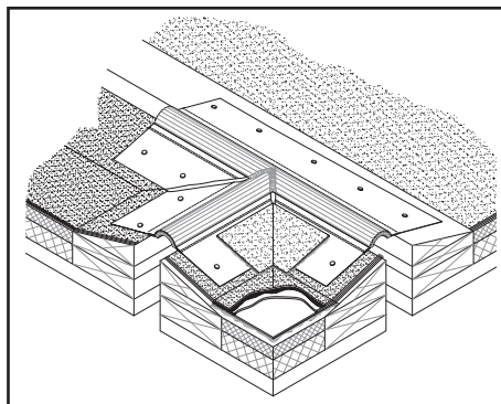
STYLE EJ PF-12 TRANSITION TEE
