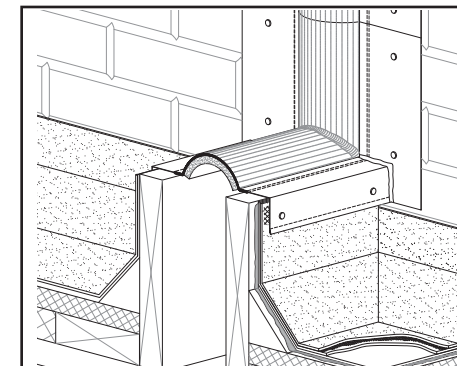
STYLE CF PF-9 TRANSITION VERTICAL INSIDE CORNER
