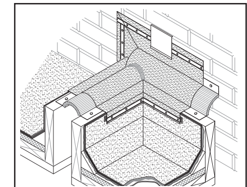
STYLE EJ/WC PF-21/25 TRANSITION ROOF/WALL TO ROOF/ROOF
