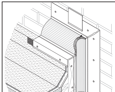
STYLE CF/EJ EG-2 TRANSITION RW VERTICAL OUTSIDE CORNER
