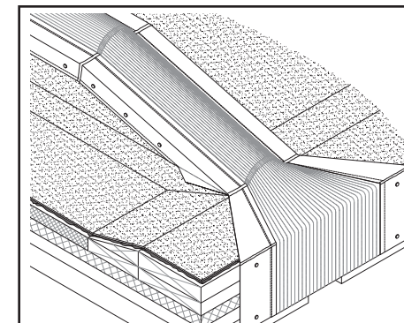
STYLE CF FF-7 TRANSITION GRAVEL STOP
