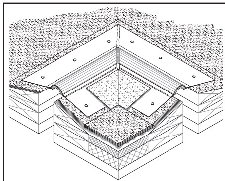
STYLE EJ PF-11 TRANSITION CORNER
