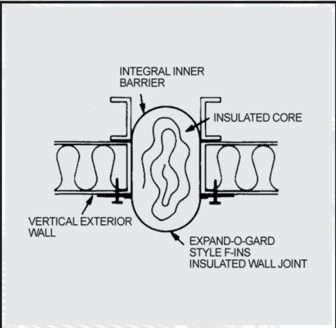
INSULATED WALL JOINT
