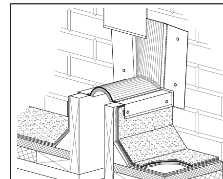
STYLE CF FF-8 TRANSITION TERMINATION
