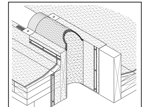
STYLE EJ/WC EG-26 TRANSITION RR VERTICAL OUTSIDE CORNER
