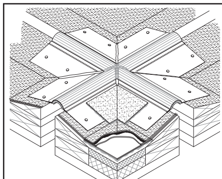
STYLE EJ PF-13 TRANSITION CROSS-OVER
