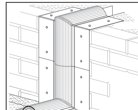
STYLE EJ PF-19 TRANSITION VERTICAL OUTSIDE CORNER
