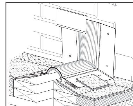
STYLE EJ FF-18 TRANSITION TERMINATION
