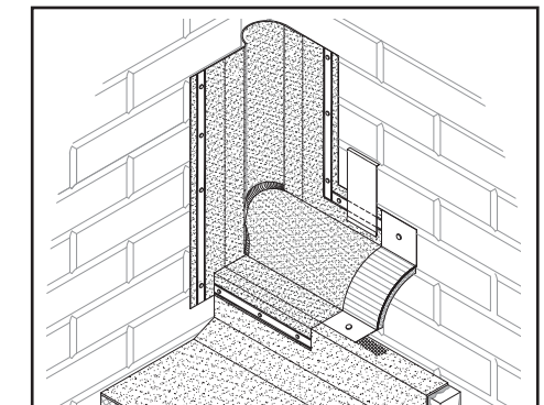
STYLE EJ/WC EG-25 TRANSITION RW VERTICAL INSIDE CORNER
