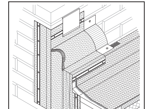
STYLE EJ/WC EG-24 TRANSITION RW VERTICAL OUTSIDE CORNER
