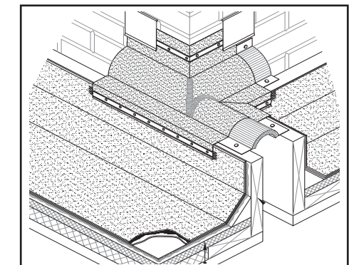
STYLE EJ/WC PF-24/26 TRANSITION ROOF/WALL TO ROOF/ROOF
