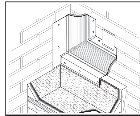
STYLE CF/EJ PF-8 TRANSITION VERTICAL INSIDE CORNER
