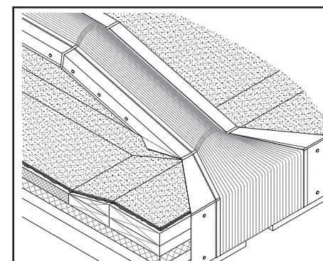
STYLE CF FF-7 TRANSITION GRAVEL STOP
