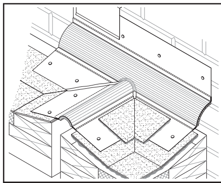
STYLE EJ PF-16 TRANSITION TEE
