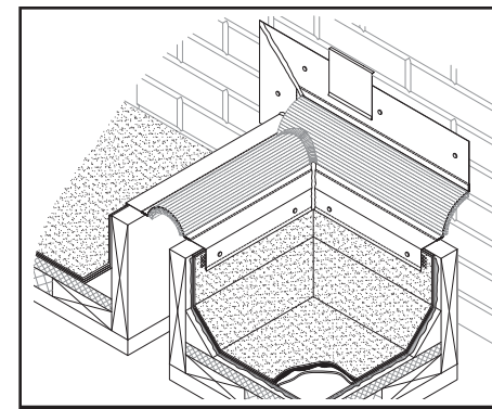
STYLE CF/EJ PF-1/5 TRANSITION ROOF/WALL TO ROOF/ROOF
