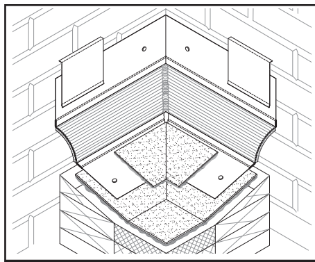
STYLE EJ PF-15 TRANSITION INSIDE CORNER
