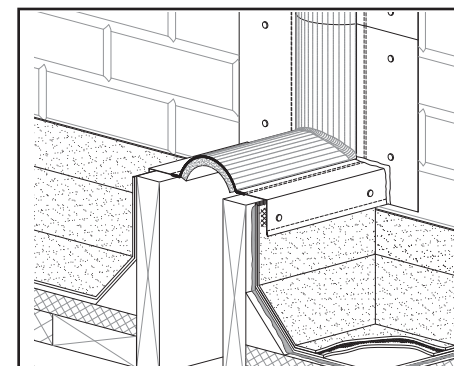
STYLE CF PF-9 TRANSITION VERTICAL INSIDE CORNER
