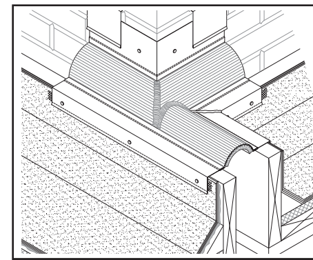
STYLE CF/EJ PF-4/6 TRANSITION ROOF/WALL TO ROOF/ROOF
