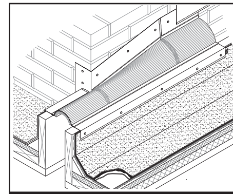
STYLE CF/EJ FF-5 TRANSITION ROOF/WALL TO ROOF/ROOF
