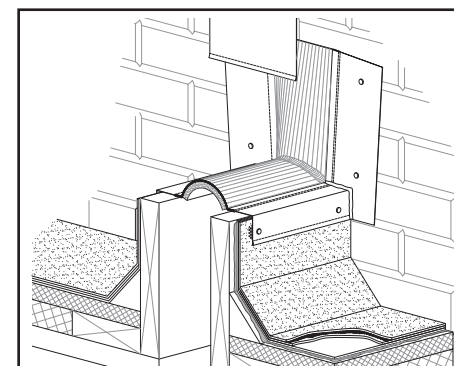
STYLE CF FF-8 TRANSITION TERMINATION
