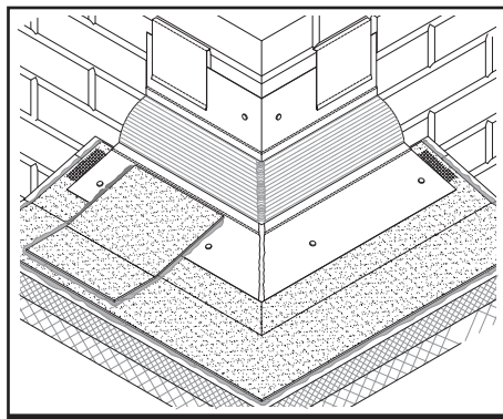
STYLE EJ PF-14 TRANSITION OUTSIDE CORNER
