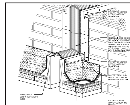
STYLE CF PF-9 TRANSITION VERTICAL OUTSIDE CORNER
