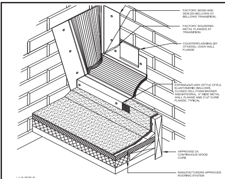
STYLE CF/EJ EW-8 RAD TRANSITION TERMINATION
