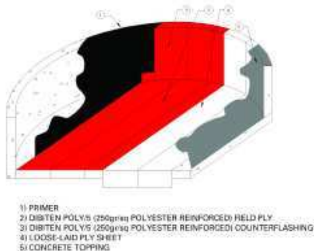
Example Above: Between-Slab Waterproofing (ex: Water Reservoirs)
