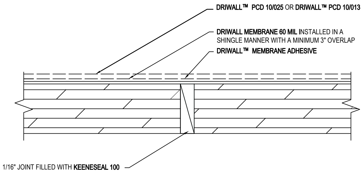
DETAIL
