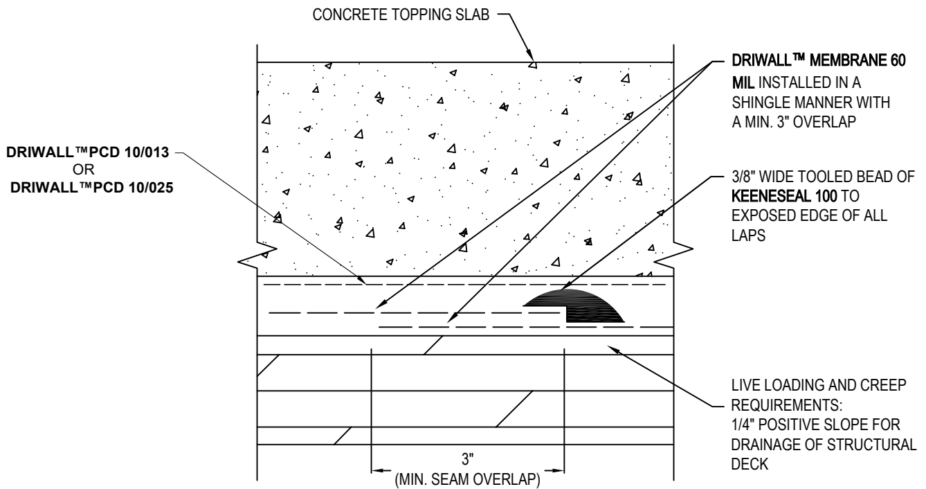
DETAIL
