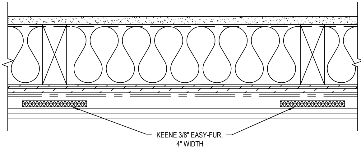
DETAIL
