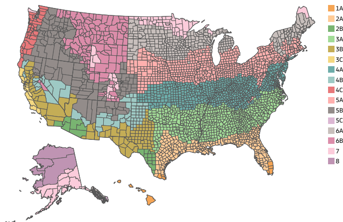
Climate Zone Map for IECC 2024
