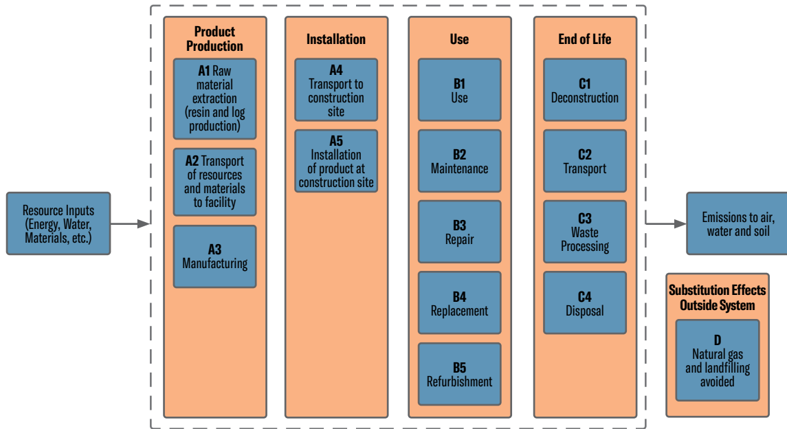
FIGURE 2 Cradle-to-Grave System Boundary for LP WeatherLogic® Air & Water Barrier
