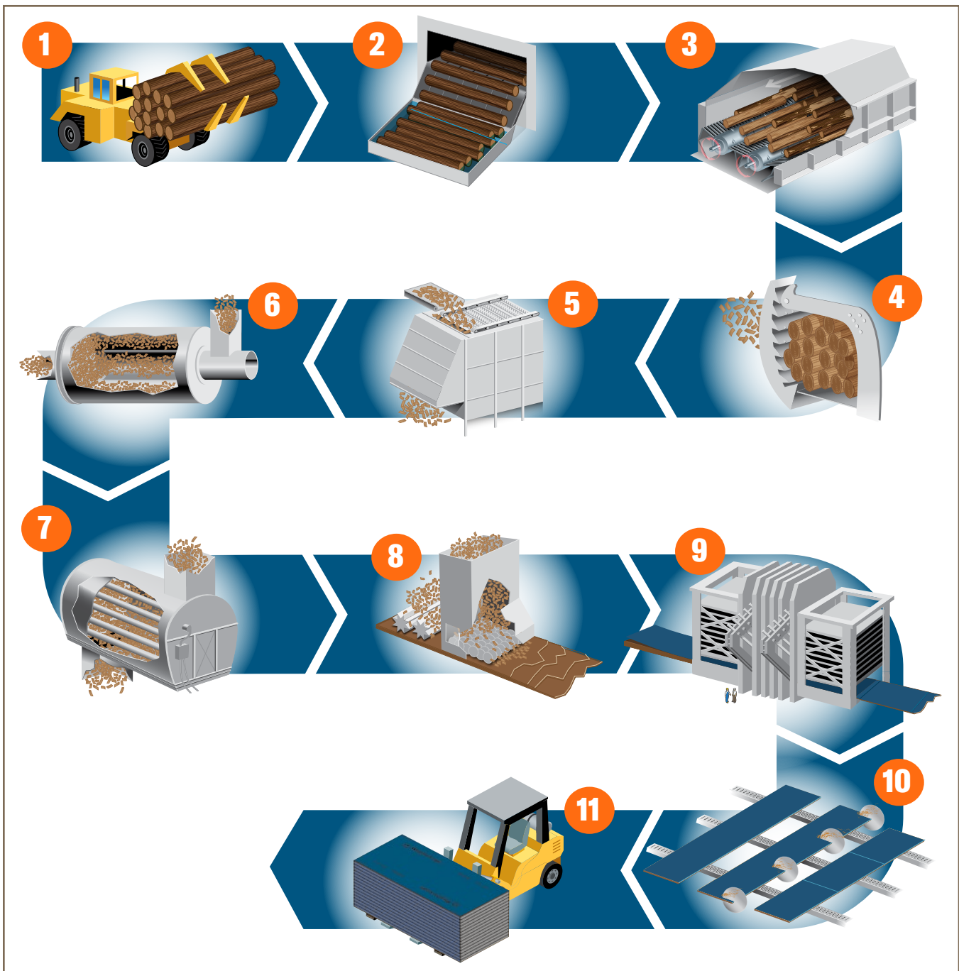
FIGURE 1 Process flow for the production of LP WeatherLogic® Air & Water Barrier
