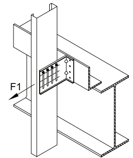
WSC600 (4 slots)
