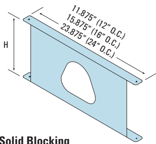
Solid Blocking
