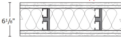
3 5/8" Wall with 2x2 Application
