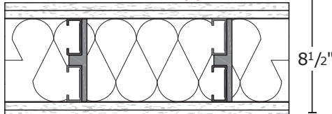
6" Wall with 2x2 Application
