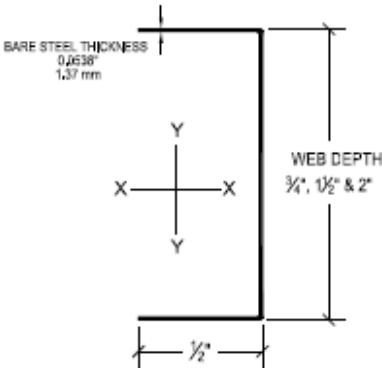
U-CHANNEL
