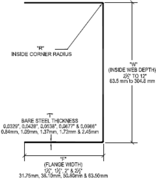
STRUCTURAL TRACK
