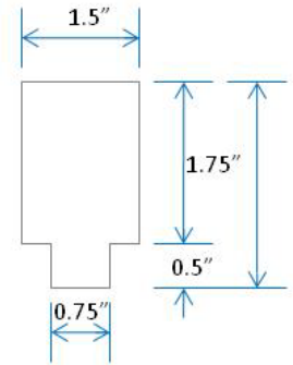
Keyhole Punch
