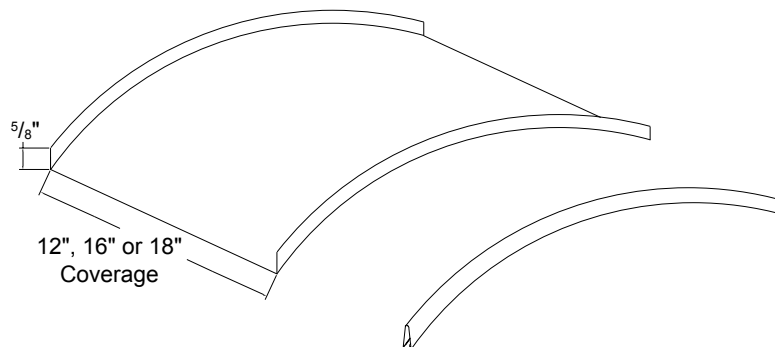
CURVED 1" MINI-BATTEN
