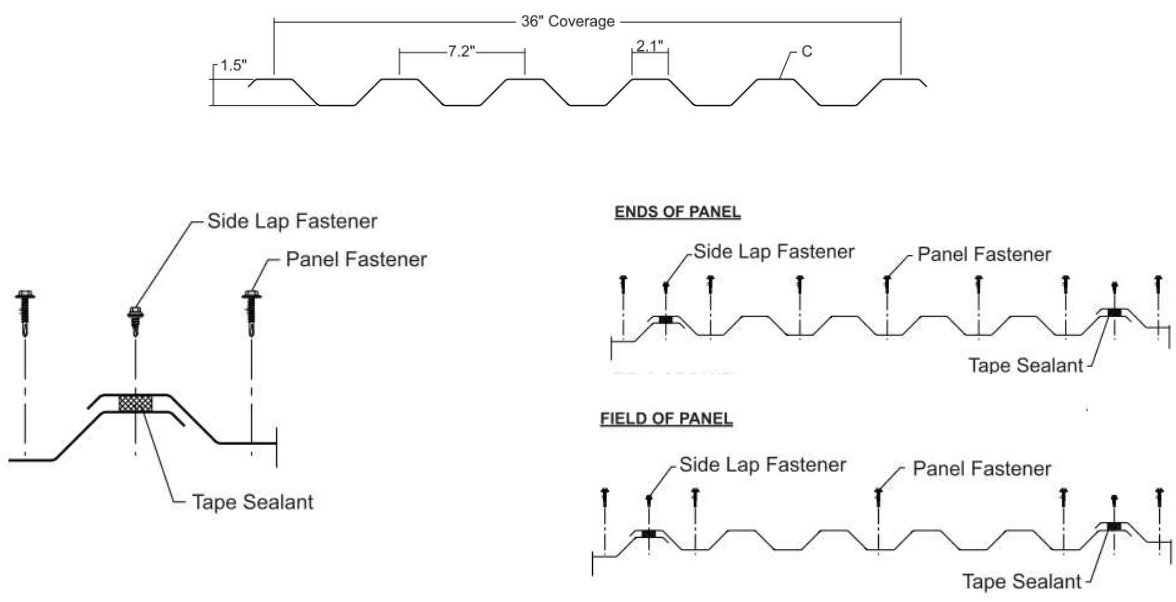
FIGURE 6—IC72 PANEL
