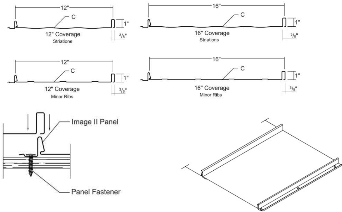
FIGURE 5—IMAGE II
