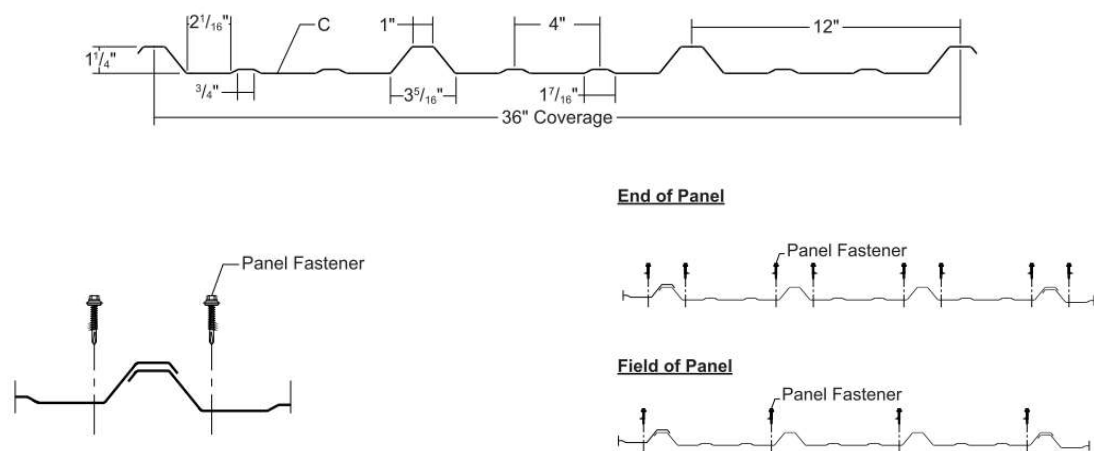
FIGURE 12—R-PANEL
