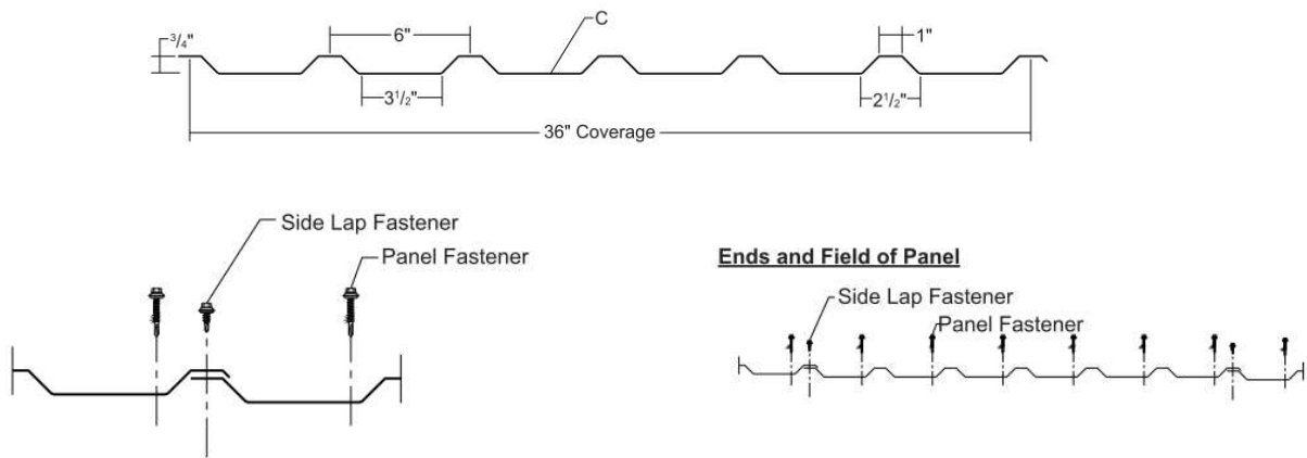
FIGURE 10—U-PANEL
