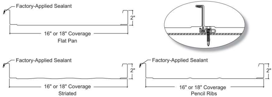
FIGURE 1A—MAGNA-LOC
