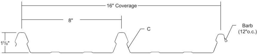
FIGURE 4A—CLIP-LOC
