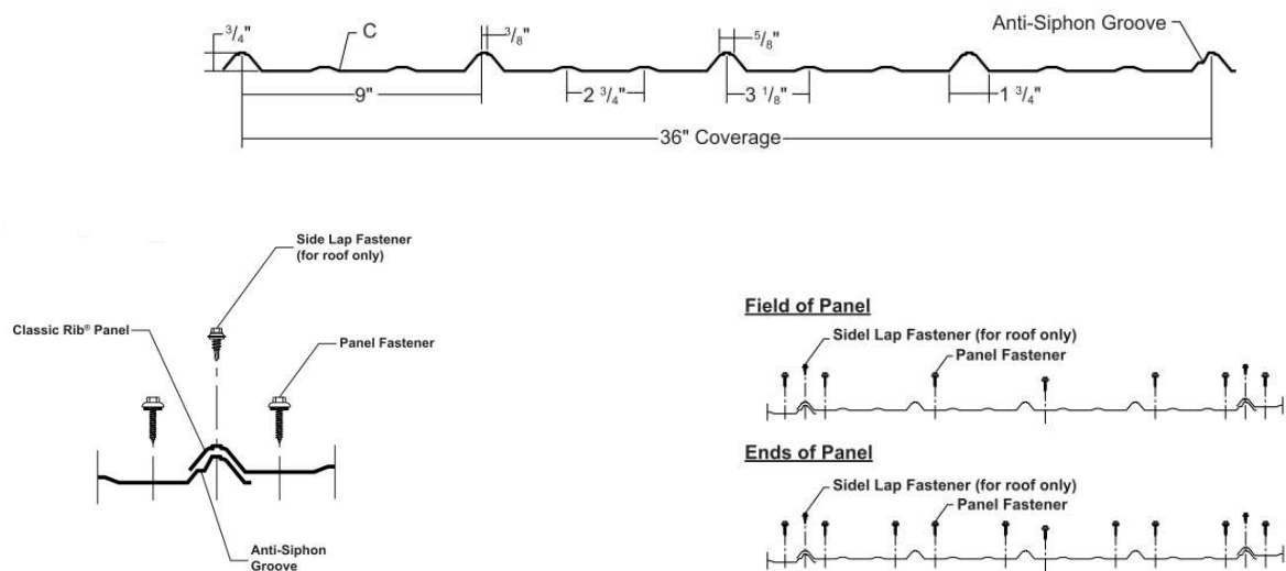
FIGURE 8—CLASSIC RIB
