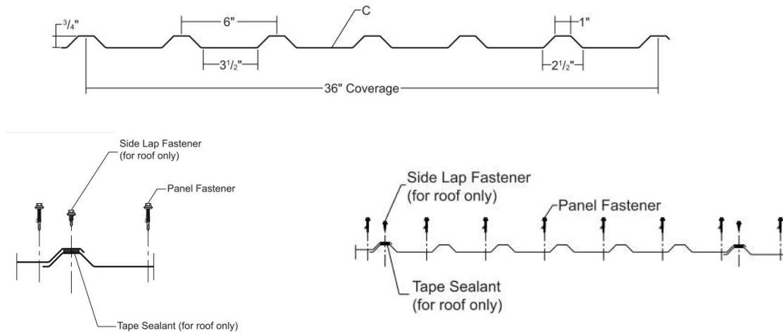
FIGURE 11—PBU-PANEL
