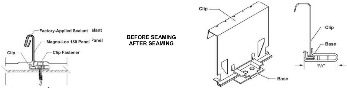
FIGURE 2B—MAGNA-LOC CLIP
