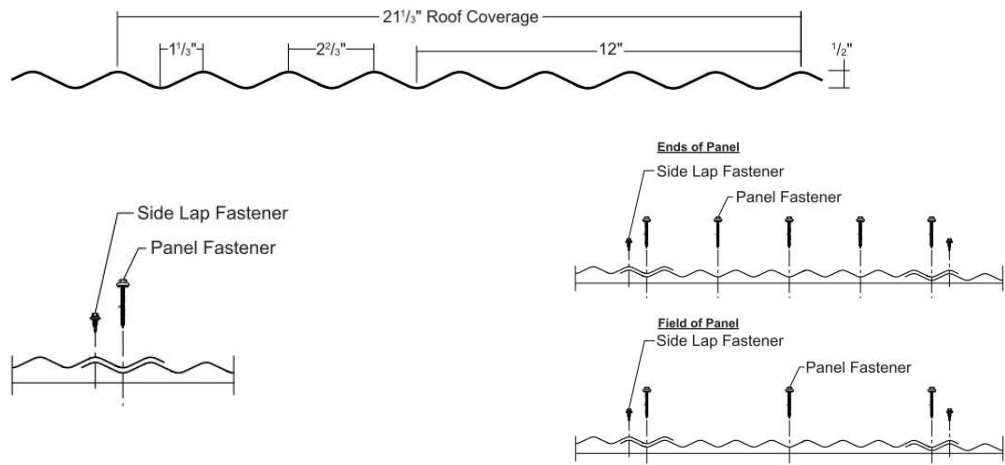
FIGURE 9—2.5" CORRUGATED
