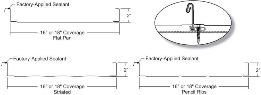
FIGURE 2A—MAGNA-LOC 180
