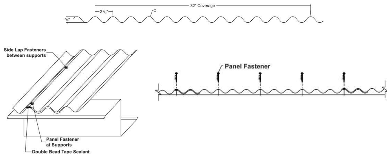
FIGURE 7—7/8" CORRUGATED
