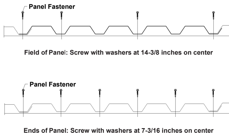
FIGURE 1—T6-A PANEL PROFILE AND FASTENING SCHEDULE FOR T6-A WALL PANELS
