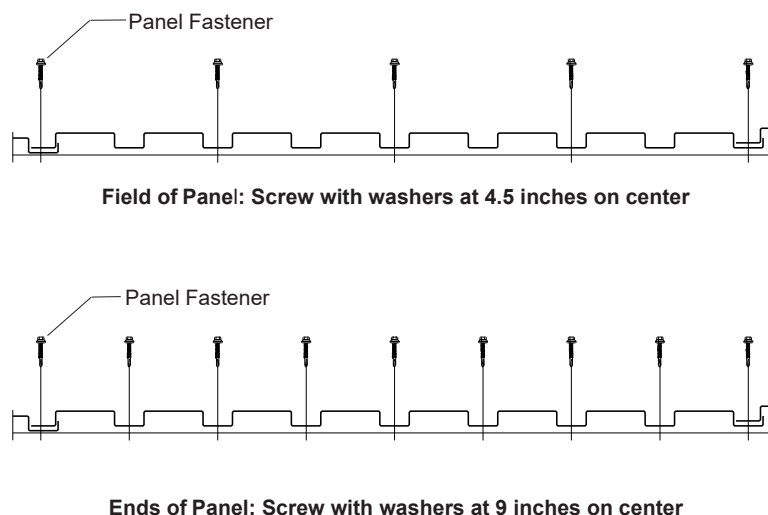
FIGURE 6—T16-E PANEL PROFILE AND FASTENING SCHEDULE FOR T16-E WALL PANELS
