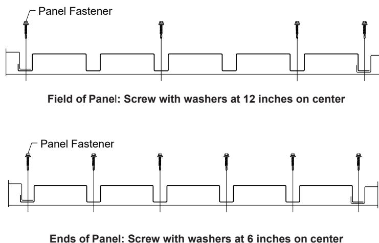
FIGURE 4—T10-C PANEL PROFILE AND FASTENING SCHEDULE FOR T10-C WALL PANELS
