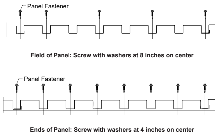
FIGURE 2—T10-A PANEL PROFILE AND FASTENING SCHEDULE FOR T10-A WALL PANELS
