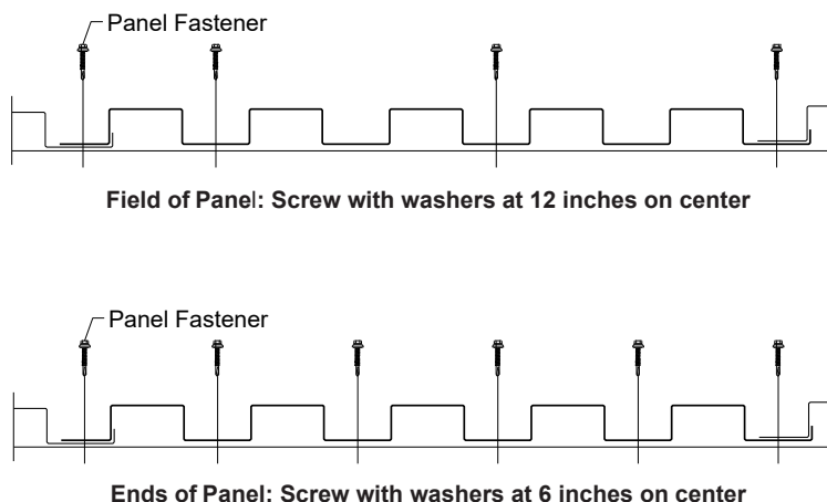
FIGURE 3—T10-B PANEL PROFILE AND FASTENING SCHEDULE FOR T10-B WALL PANELS
