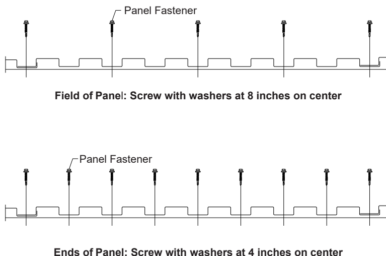
FIGURE 7—T16-L PANEL PROFILE AND FASTENING SCHEDULE FOR T16-L WALL PANELS
