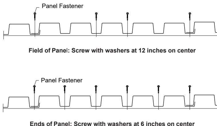
FIGURE 9—T2630 PANEL PROFILE AND FASTENING SCHEDULE FOR T2630 WALL PANELS
