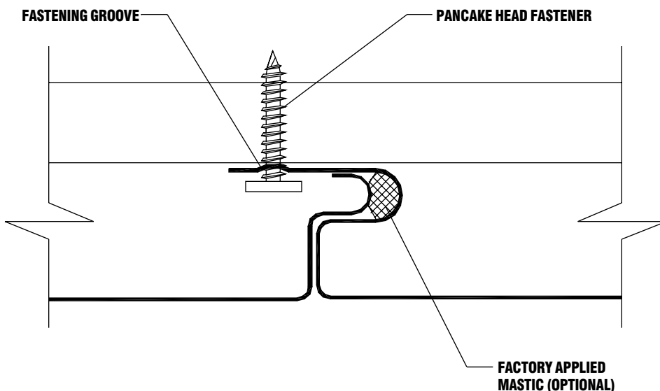
INSTALLED PANEL CROSS SECTION
