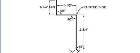
Translucent Panels
