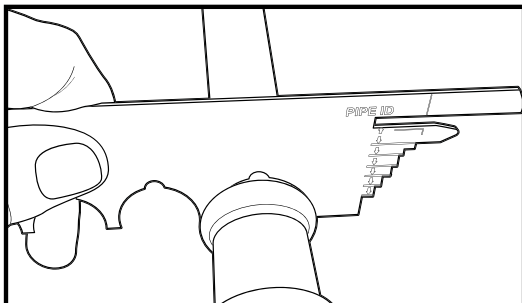
Streamline® ACR Press Fitting Insertion Depth Chart (1/4" to 1-3/8")
